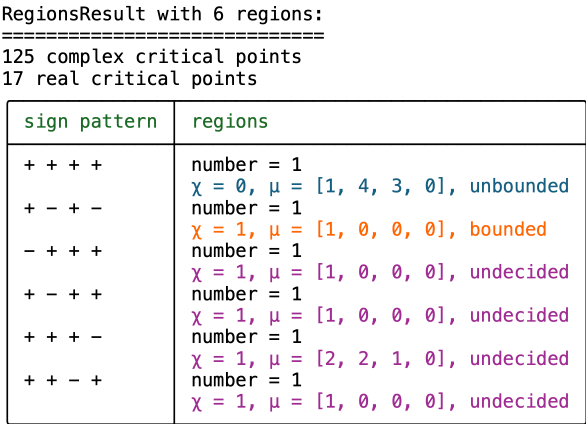
Figure 6. Output of HypersurfaceRegions.jl for four paraboloids in \mathbb{R}^3 .
